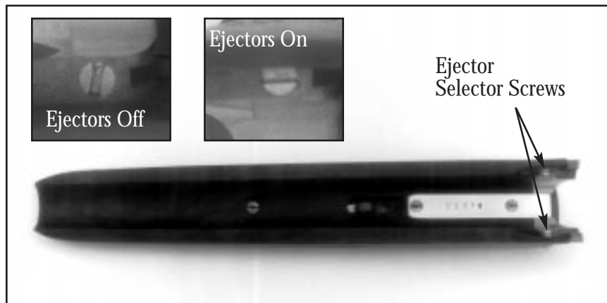
Figure 4 - Disconnectable Ejectors
