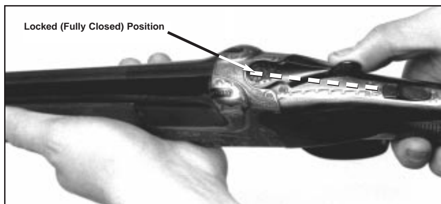
Figure 5 -Closing the Breech
