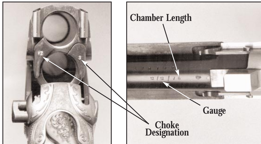
Figure 8 - Gauge, Chamber Length and Choke Designation
