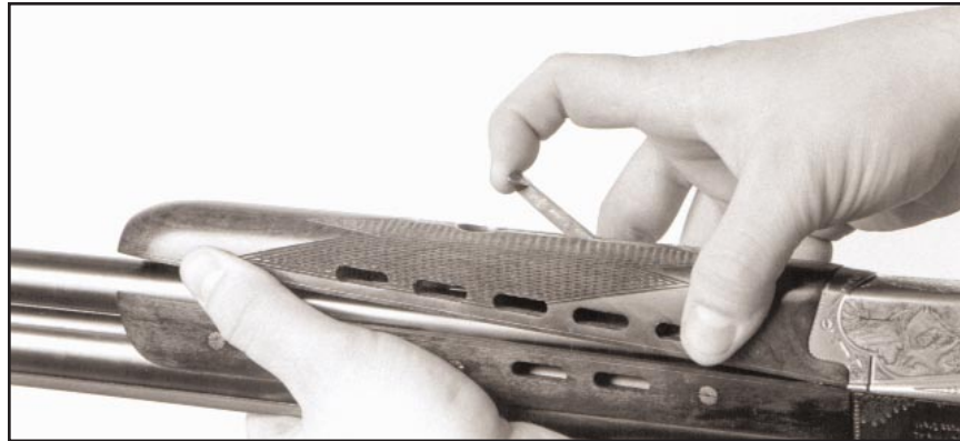
Figure 6 - Removal of Forearm
